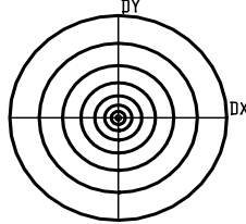
Third-order spherical aberration
