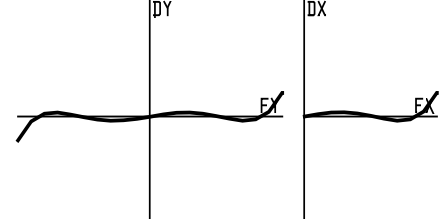
Balanced third + fifth + focus
