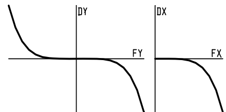
Fifth-order spherical aberration
