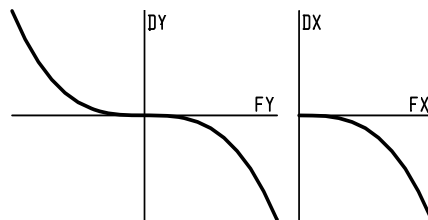
Third-order spherical aberration
