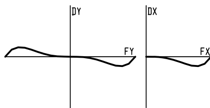
Balanced third + fifth spherical
